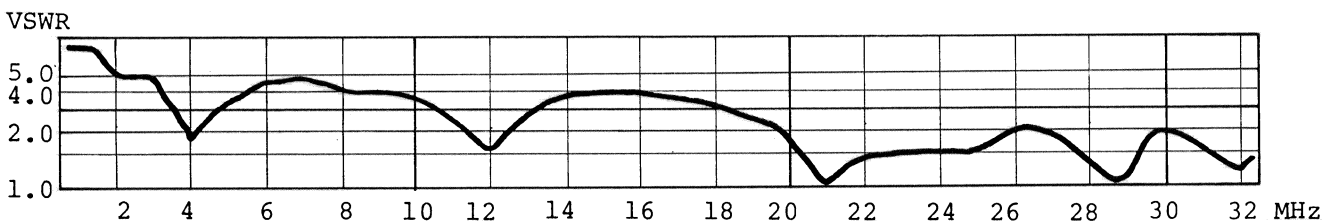
WD230-1 VSWR Curve, Typical
