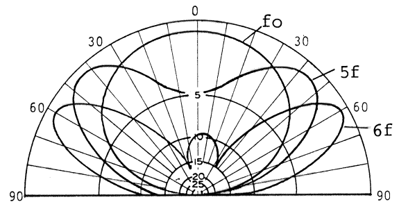
Azimuth Pattern, fo, 5f, 6f
