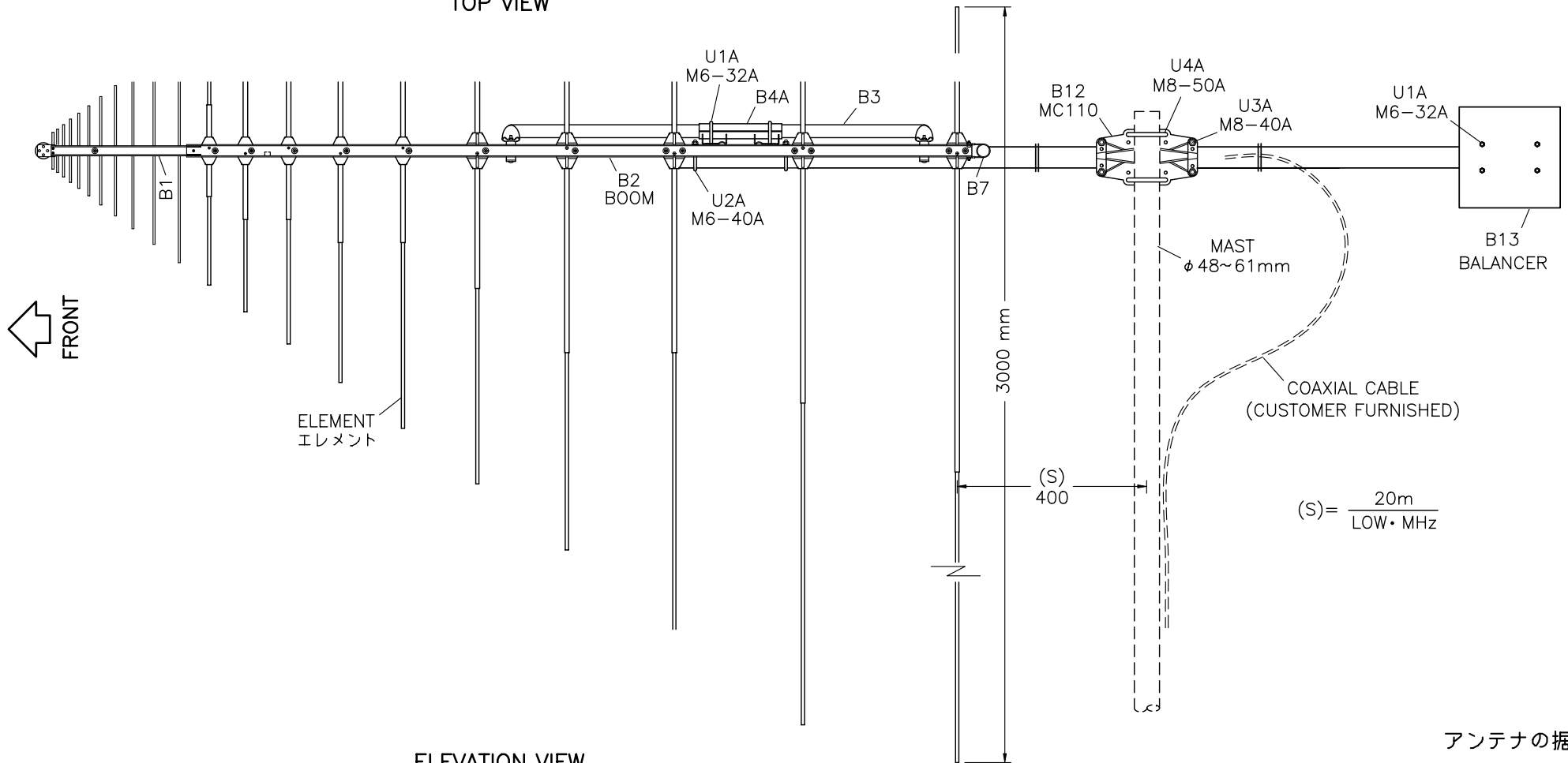
Figure 3A. CLP5130-1D, Antenna Installation.
